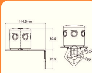
Sidewall Type
