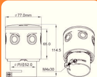
Sleeve Type
