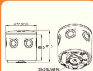
Magnetic suction Type
